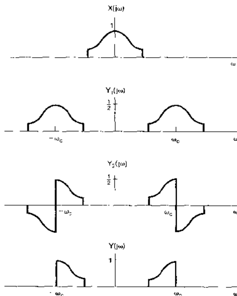
Figure 8.22 Spectra associated with the single-sideband system of Figure 8.21
