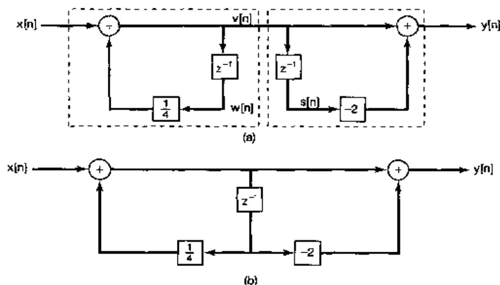
Figure 10.19 (a) Block-diagram representations for the system in Example 10.29; (b) equivalent block-diagram representation using only one unit delay element.
