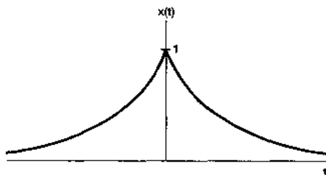
Figure 4.6 Signal x(t) = e^{-a|t|} of Example 4.2
